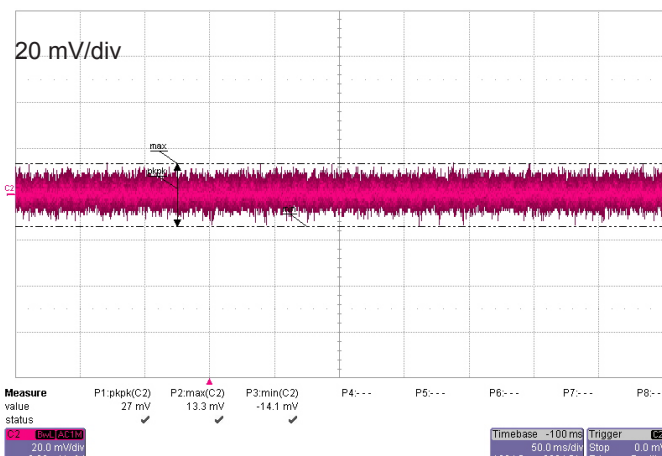
Figure 15: Output noise
