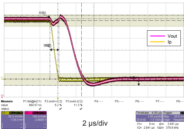
Figure 13: Step response
