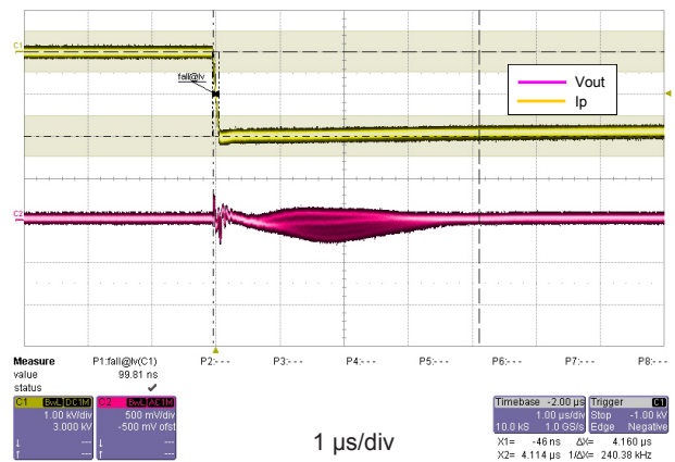
Figure 14: dv/dt
